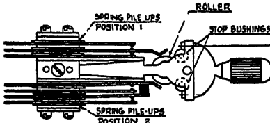
Lever switching key.
